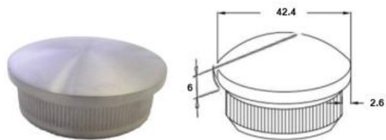
EK1010K-42.4 Convex End Cap 304/316
