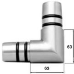
RV1005 90 Degree Sharp Bend 304
