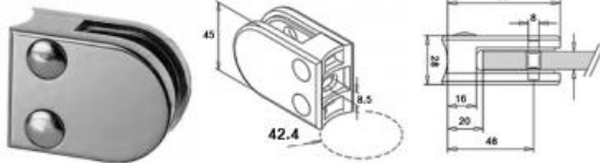
KLH10 D-Shape Glass Clamp
