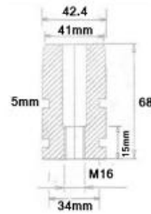
BDH1005-120x3-42.4 Smaller 68mm Spigot x 120mm Plate 304/316
