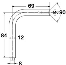
KT-Twist-Lock-90mm 90mm Off-Set Twist and Lock Handrail Bracket
