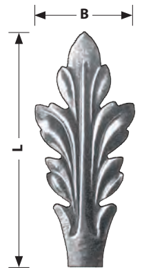
L: 110 mm B: 45 mm FA 110 L: 4 5/16" B: 1 3/4" L: 180 mm B: 79 mm FA 180 L: 7 1/16" B: 3 1/8"
