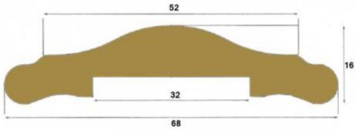
N-24662 - Unpolished Brass Handrail N-24662-P - Polished Brass Handrail
