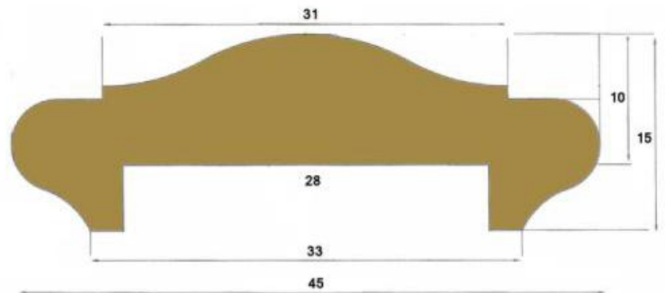
N-00015 - Unpolished Brass Handrail N-00015-P - Polished Brass Handrail
