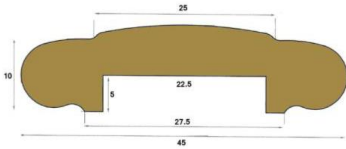
N-00013 - Unpolished Brass Handrail N-00013-P - Polished Brass Handrail
