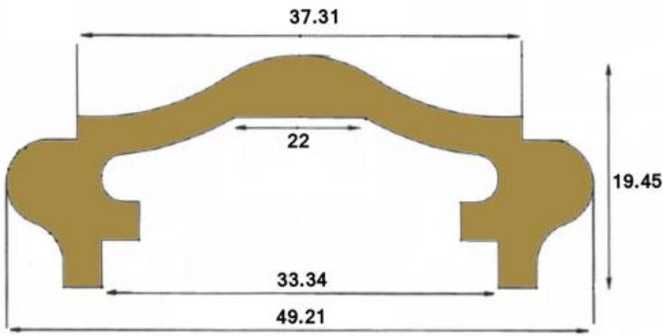
N-23400 - Unpolished Brass Handrail N-23400-P - Polished Brass Handrail
