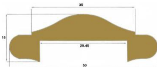
N-25920 - Unpolished Brass Handrail N-25920-P - Polished Brass Handrail
