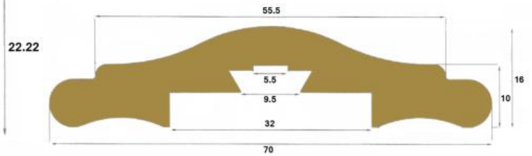
N-24051 - Unpolished Brass Handrail N-24051-P - Polished Brass Handrail
