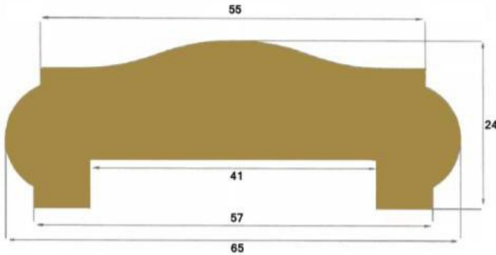
N-26692 - Unpolished Brass Handrail N-26692-P - Polished Brass Handrail
