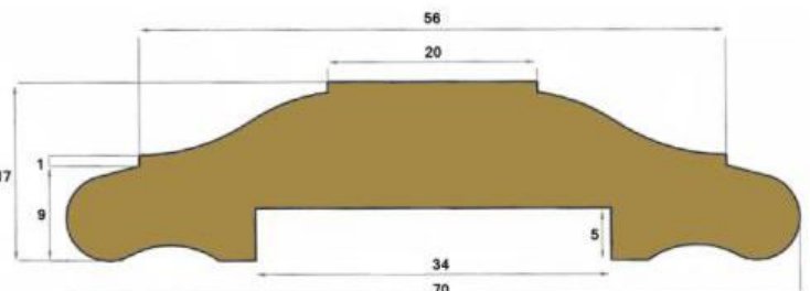
N-05241 - Unpolished Brass Handrail N-05241-P - Polished Brass Handrail
