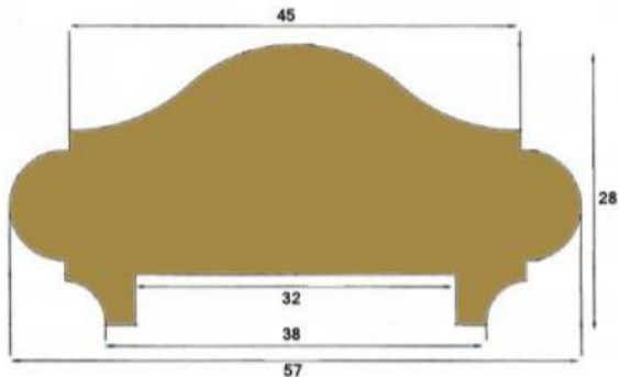
N-25629 - Unpolished Brass Handrail N-25629-P - Polished Brass Handrail
