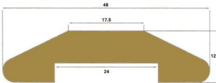
N-00041 - Unpolished Brass Handrail N-00041-P - Polished Brass Handrail
