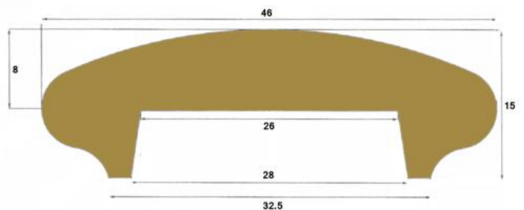
N-24147 - Unpolished Brass Handrail N-24147-P - Polished Brass Handrail
