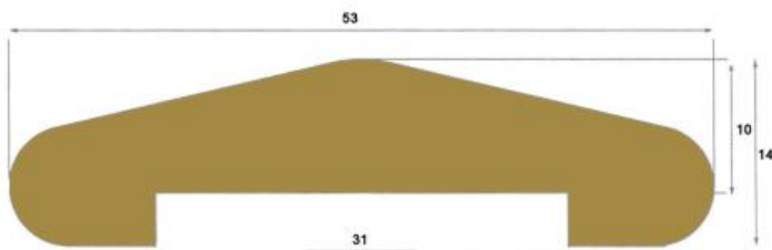
N-24127 - Unpolished Brass Handrail N-24127-P - Polished Brass Handrail
