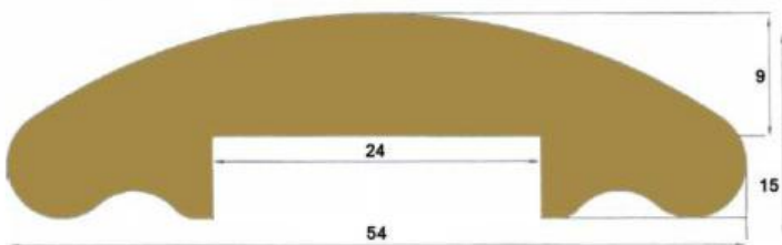
N-01209 - Unpolished Brass Handrail N-01209-P - Polished Brass Handrail
