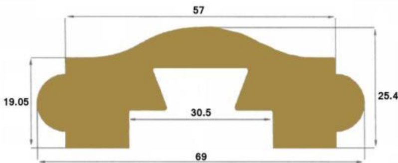
N-26755 - Unpolished Brass Handrail N-26755-P - Polished Brass Handrail
