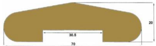
N-25901 - Unpolished Brass Handrail N-25901-P - Polished Brass Handrail
