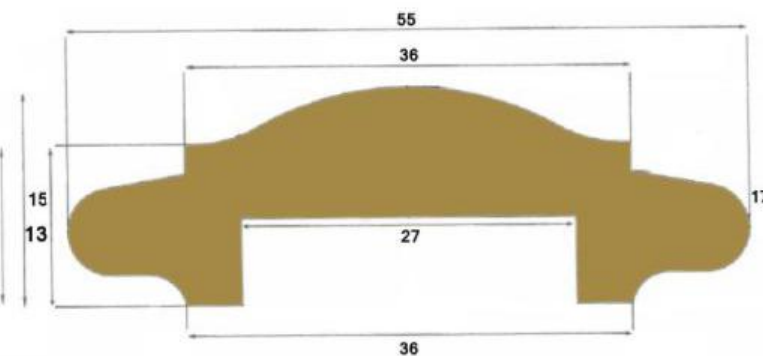
N-21939 - Unpolished Brass Handrail N-21939-P - Polished Brass Handrail
