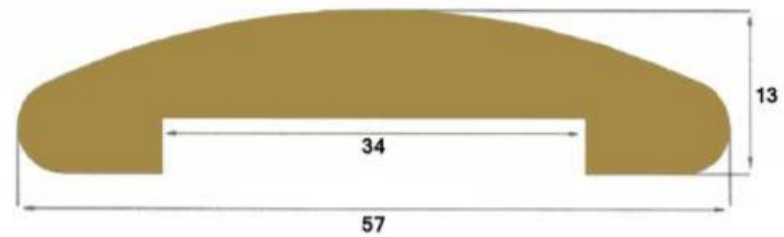
N-26699 - Unpolished Brass Handrail N-26699-P - Polished Brass Handrail
