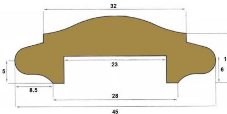
N-21880 - Unpolished Brass Handrail N-21880-P - Polished Brass Handrail
