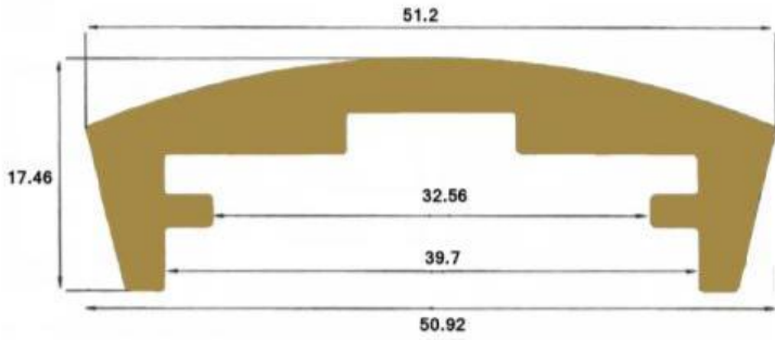
N-26025 - Unpolished Brass Handrail N-26025-P - Polished Brass Handrail
