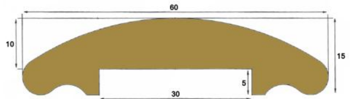
N-23782 - Unpolished Brass Handrail N-23782-P - Polished Brass Handrail
