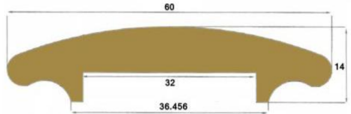
N-24663 - Unpolished Brass Handrail N-24662-P - Polished Brass Handrail
