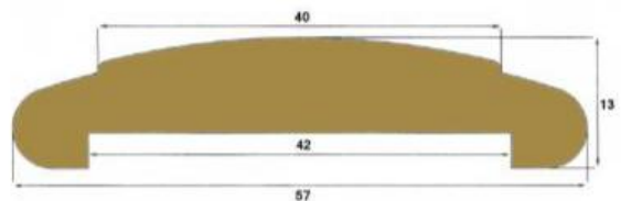
N-26018 - Unpolished Brass Handrail N-26018-P - Polished Brass Handrail
