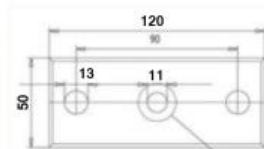
RON1007K M10 - 120 x 50mm / M16 - 140 x 60mm 304/316
