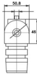
GLS1001K-316-50.8 Adjustable Angle Insert
