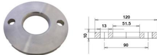
RON1010/50.8 Weldable Plate 304/316
