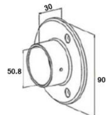
WALLPLATE-50.8 Wall Plate with 3 x M6 Fixing Holes 316
