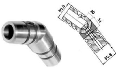
RV1011-50.8 0-40 Degree Angle Changer
