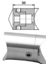
RA1010 50/50mm Connector 304
