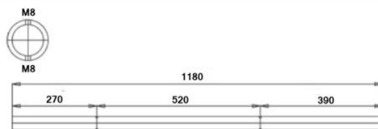
SP1002 - 1180mm High Mid Post 4 x M8 pre-drilled holes by 180 degrees. Holes at 520mm c/c
