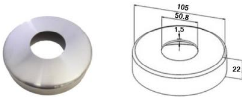
ROS1001-50.8 Cover Plate 304/316
