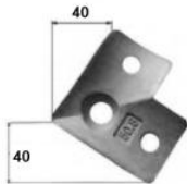
HH1001K-Z-50.8 90 Deg Angle Saddle 316
