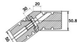
RA1006/50.8 Adaptor 50.8 Ali Insert 304/316
