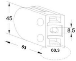
KLH10D-60.3 Glass Clamp + 10mm Rubber Inserts (Rubbers Also Available for 6/8/12mm Glass) 316 Satin
