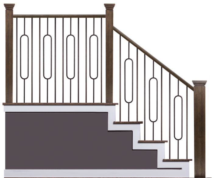
HF-16.1.32 Ends: 12 mm Sq. Height: 1117mm Weight: 4.55kg
