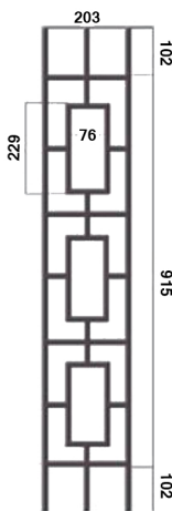
HF-9.4.3 Ends: 12mm Sq. Height: 1119mm Weight: 2.27kg
