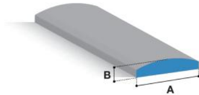
KT-1187 A = 50mm B = 12mm
