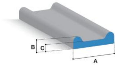
KT-1294 A = 25mm B = 8mm C = 4mm
