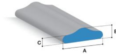
KT-2505 A = 50.8mm B = 15.4mm C = 9mm
