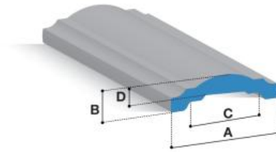
KT-1346 A = 50mm B = 13mm C = 33mm D = 7.5mm
