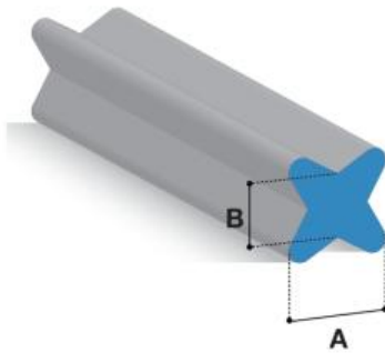
KT-1110A A = 15mm B = 9mm
