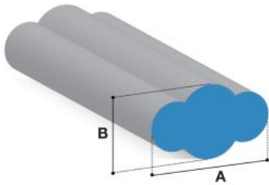
KT-1263 A = 20.5mm B = 12mm
