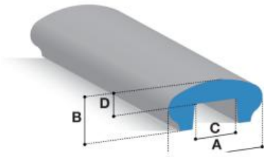
KT-1356 A = 40mm B = 18mm C = 18mm D = 8mm KT-1411 A = 50mm B = 22.5mm C = 18mm D = 10mm
